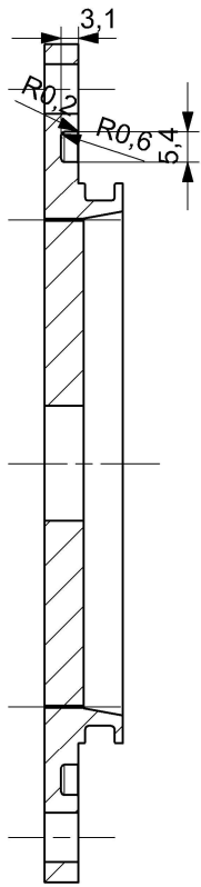
SECTION C-C
